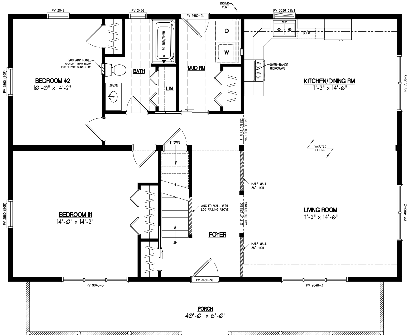
30x44 MOUNTAINEER DELUXE Plan #30MD1404
